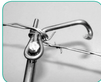
Turn Tool Handle
